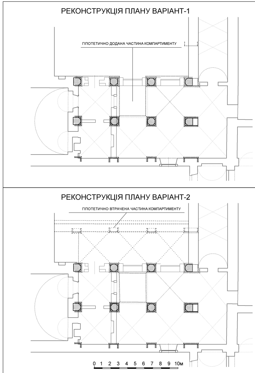
. 2. ( 2 – ). Fig. 2. Two variants of graphic reconstruction of researched object (variant 2 – with reconstruction of lost part of kompartment).
